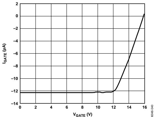
Figure 11. Gate Pull-Up Current vs. Gate Voltage at V CC = 5 V
