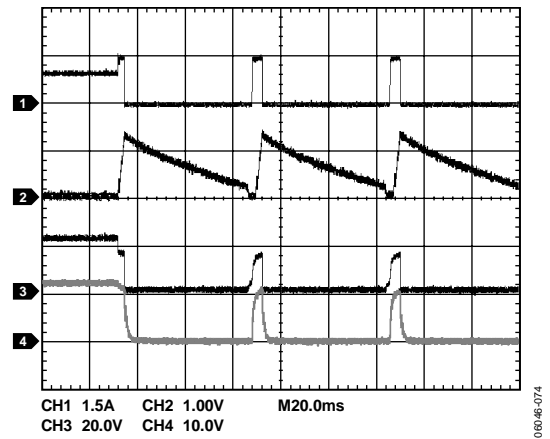
Figure 45. Overcurrent Condition During Operation (ADM1176-2 Model) (CH1 = I_{LOAD} , CH2 = V_{TIMER} , CH3 = V_{GATE} , CH4 = V_{OUT} )
