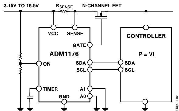
Figure 2. Applications Diagram
