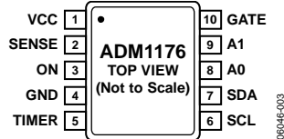
Figure 3. Pin Configuration
