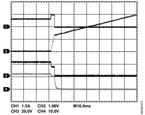
Figure 44. Overcurrent Condition During Operation (ADM1176-1 Model) (CH1 = I_{LOAD} , CH2 = V_{TIMER} , CH3 = V_{GATE} , CH4 = V_{OUT} )
